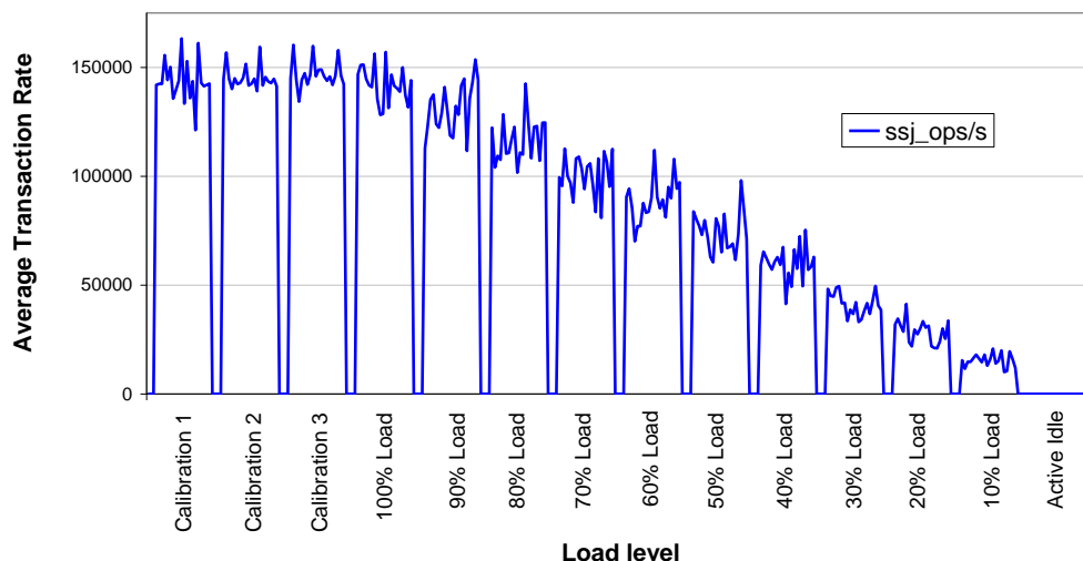
Graduated Load Levels during a Compliant Benchmark Run
