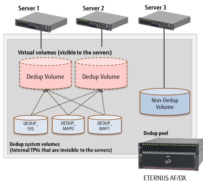
Figure 5 Configuration management of the Deduplication/Compression function
